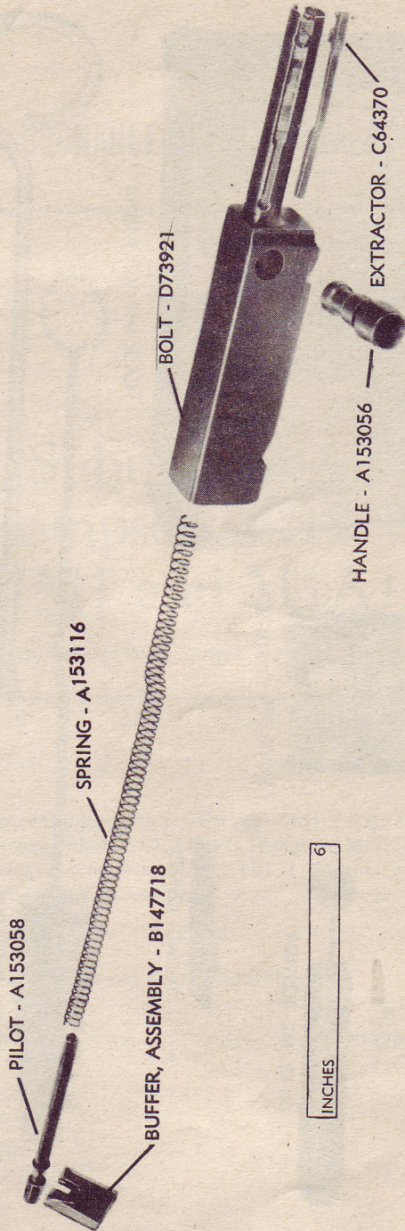
RA PD 82780 Figure 13 — Bolt and Spring Group Parts for Gun, Submachine, Cal. .45, Thompson, M1A1
