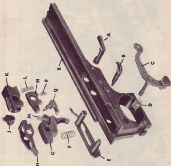
Figure 6 — Frame Group Parts for Gun, Submachine, Cal. .45, Thompson, M1928A1
