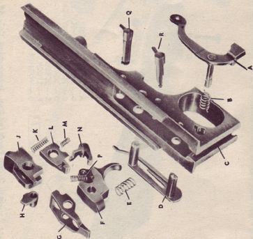
Figure 10 — Frame Group Parts for Gun, Submachine, Cal. .45, Thompson, M1 and M1A1
